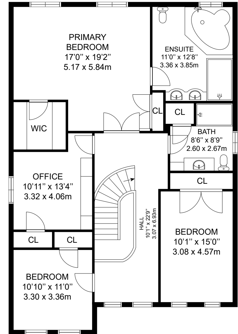
FLOOR 3
